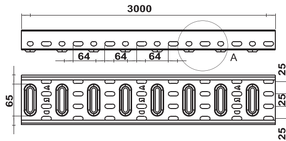
Technical drawing of AYN-10-40-07
