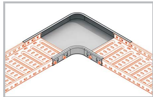
120-4 Connection Example
